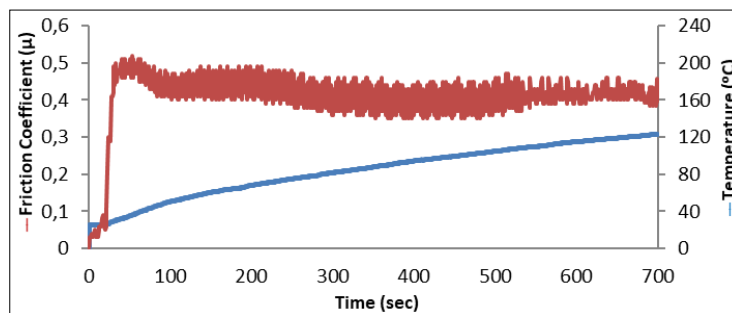
Fig 3: Time dependent friction coefficient graph of sample containing 6% nano graphite
