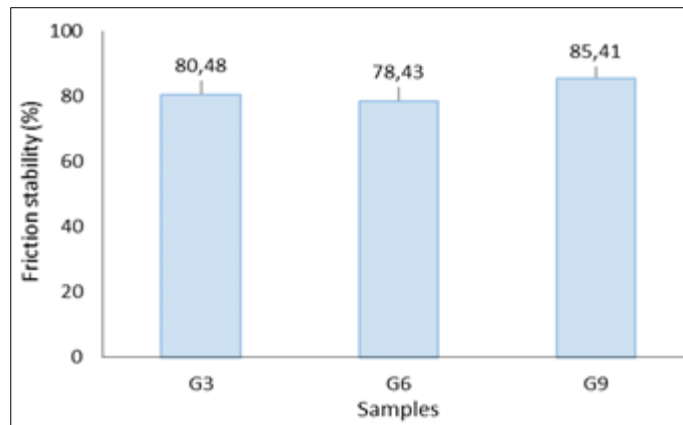
Fig 5: Friction stability of samples containing nano graphite (%)
