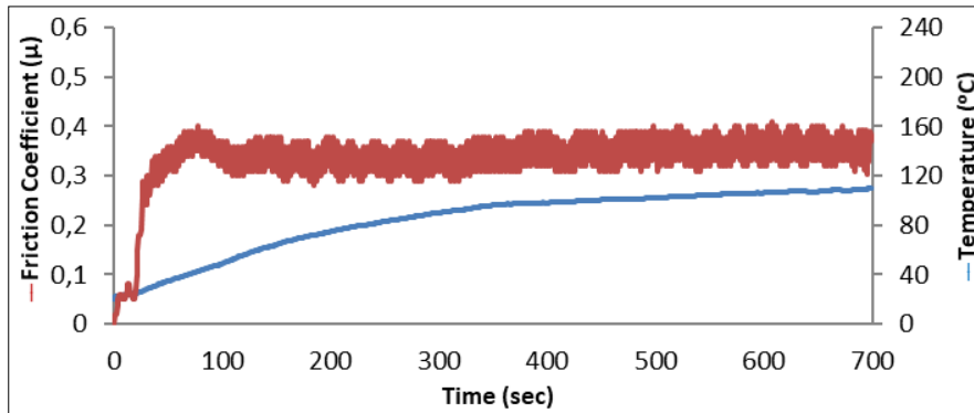
Fig 2: Time dependent friction coefficient graph of sample containing 3% nano graphite
