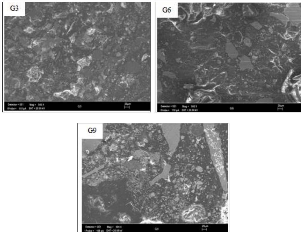
Fig 6: SEM morphologies of frictional surface of G3, G6 and G9 coded samples
