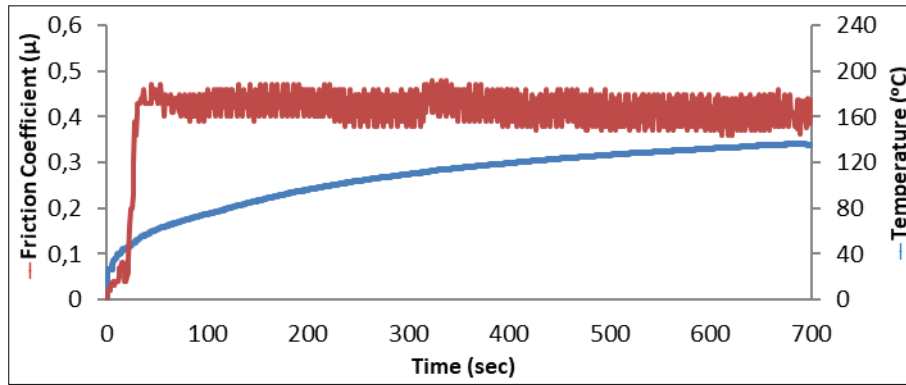
Fig 4: Time dependent friction coefficient graph of sample containing 9% nano graphite
