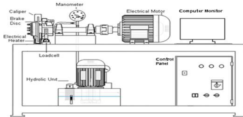
Fig 1: The brake lining test device [9]
