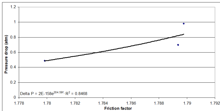
Fig 1: Pressure drop of bed versus friction factor.
