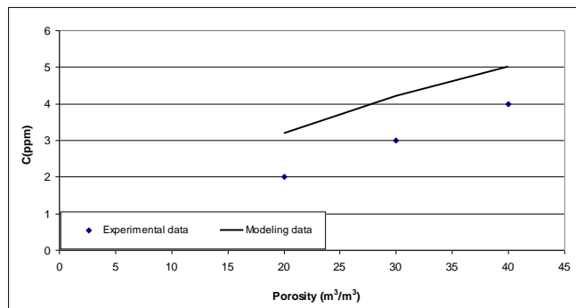
Fig 2: The effect of porosity on outlet hydrogen sulfide.
